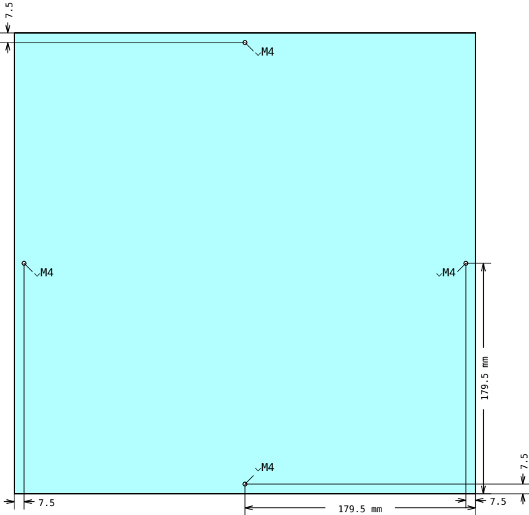
DRAWING 1, Pos 3 Hole placement
