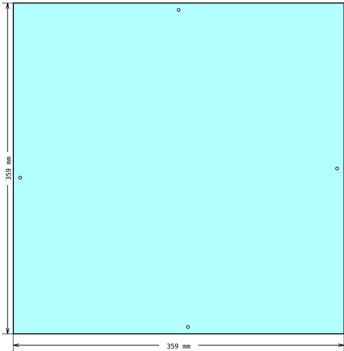
DRAWING 2, Pos 4 Shape measurements
