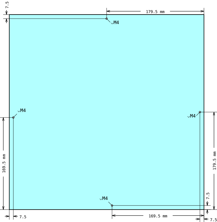
DRAWING 2, Pos 4 Hole placement
